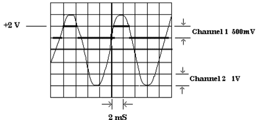
Figure 4. Remote trigger level - +2 V.
