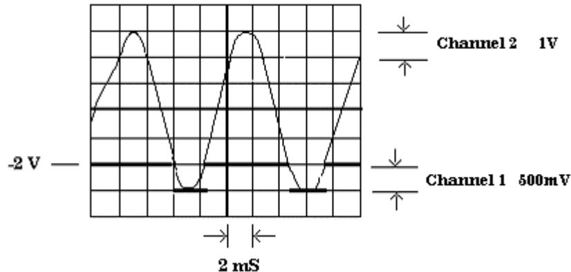
Figure 5. Remote trigger level - 2 V.
